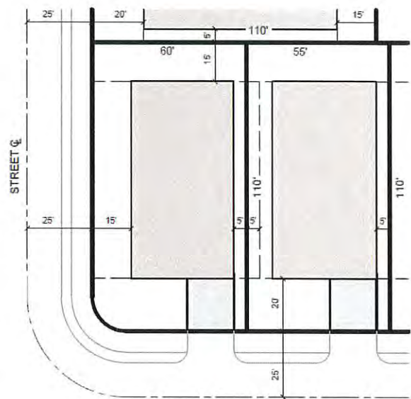
50' R/W DIAGRAM
